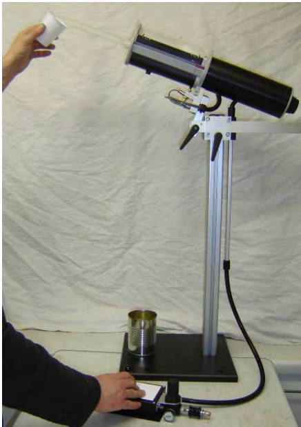
Multi axis adjustable gun support stand
