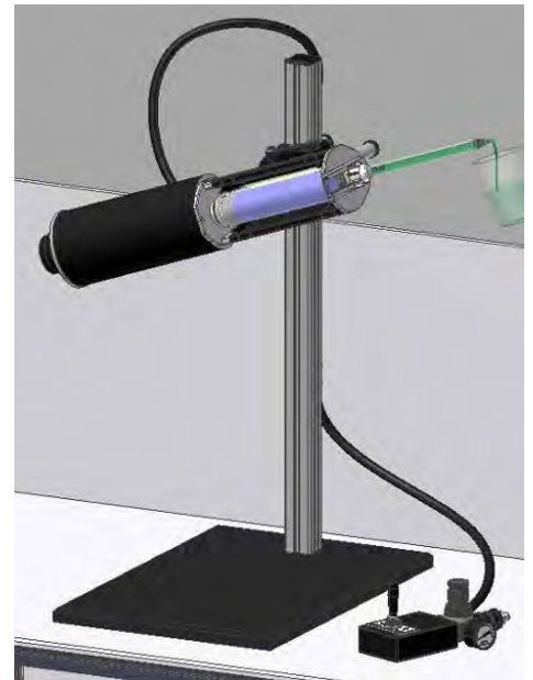
Swivel facility to prime mixer
