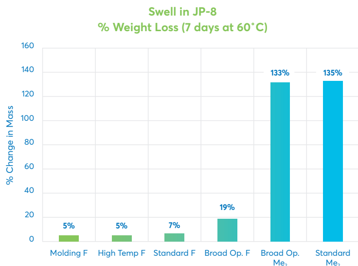
FIGURE 3: Four NuSil fluorosilicones and two dimethyl silicone materials were subjected to a swell test. All cured samples were submerged in JP-8 jet fuel for seven days at 60°C.
